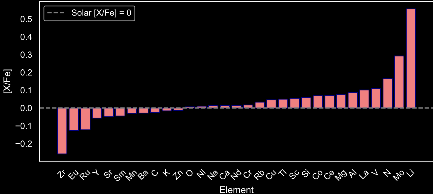
Abundance Pattern for GALAH Main Sequence Stars: Star Field [40] (N=118)
