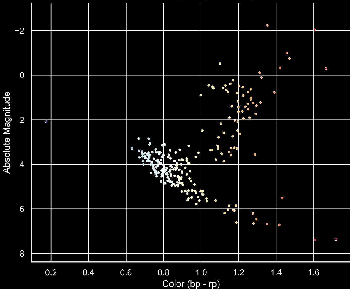
GALAH Hertzsprung-Russel Diagram Field [40] Ra [323.38] Dec [-22.42]
