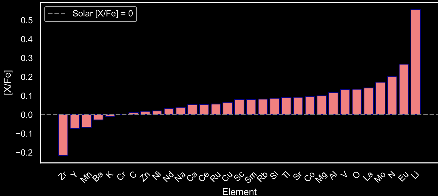
Abundance Pattern for GALAH Star Field [40] (N=247)
