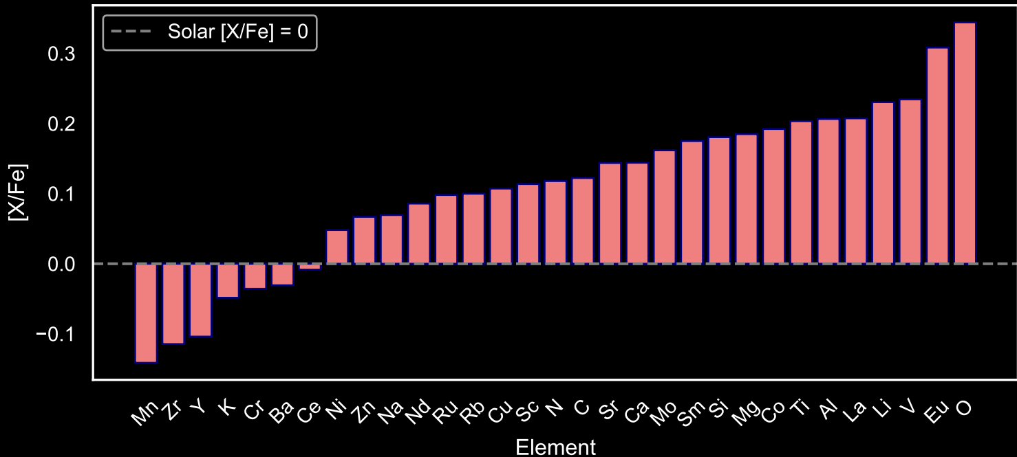
Abundance Pattern for GALAH Red Giants: Star Field [40] (N=56)
