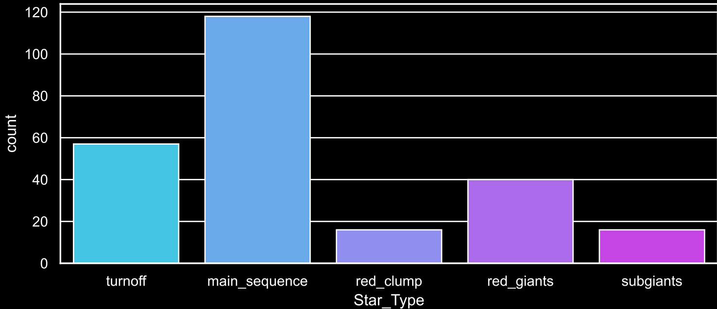
Field [40] Count plot of Star Type
